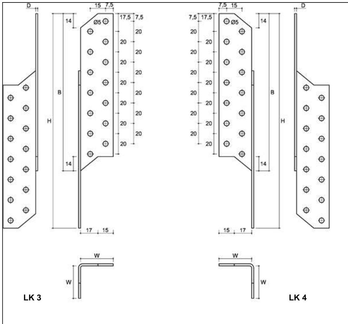
Figure 78 Type LK
