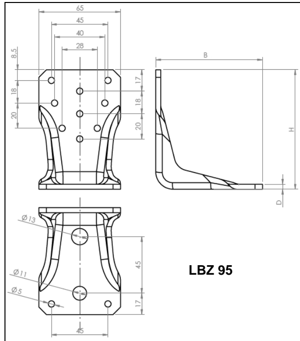
Figure 74 Type LBZ
