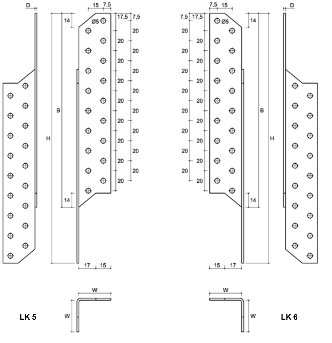
Figure 79 Type LK
