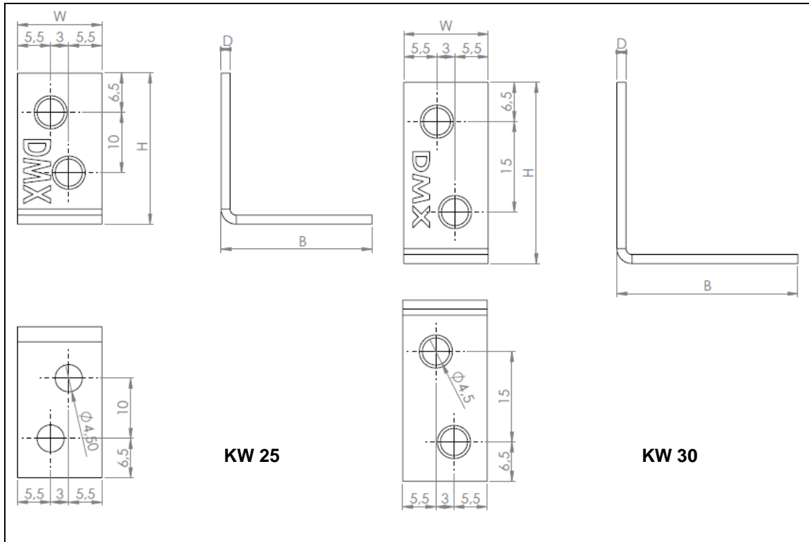
Figure 67 Type KW
