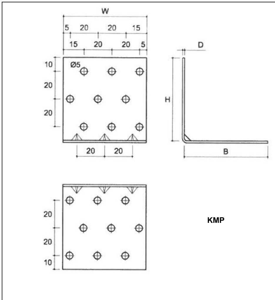
Figure 42 Type KMP
