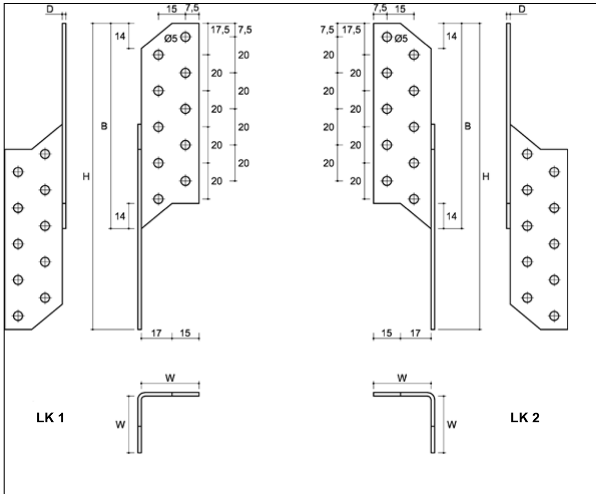
Figure 77 Type LK
