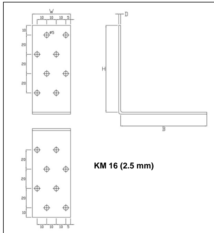
Figure 35 Type KM
