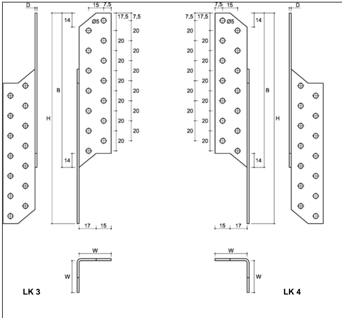
Figure 78 Type LK
