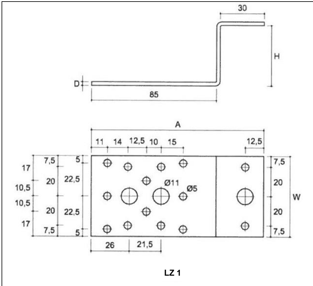
Figure 11 Type LZ
