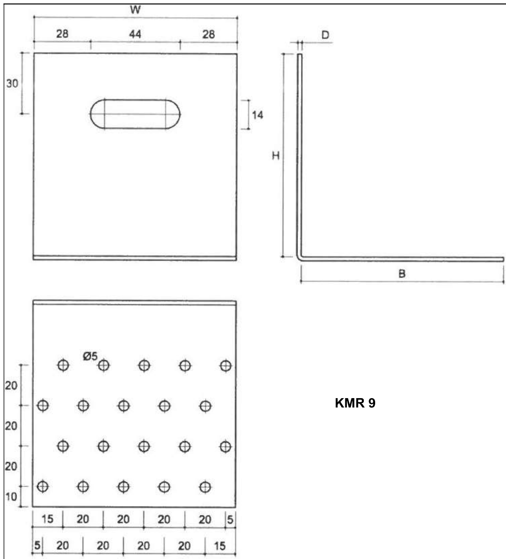
Figure 47 Type KMR
