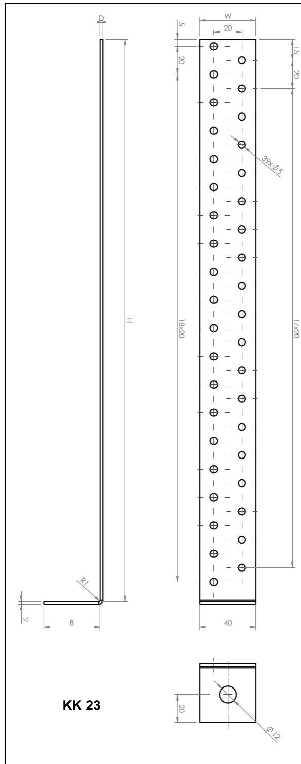
Figure 17 Type KK
