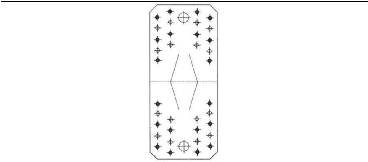
Figure 150 Type KP 2 and KPL 2
